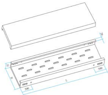
托盘式直通桥架 XQJ-P1-01 Tray Type Straight Cable Tray Model XQJ-P1-01
