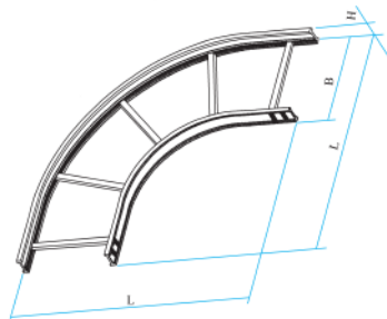
XQJ-LQJ-RT型水平弯通 LQJ-RT Horizontal Elbow
