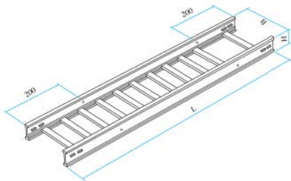
XQJ-LQJ-T型梯级式桥架 LQJ-T Ladder Frame
