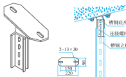
XQJ-H-03C槽钢倾斜底座 Trough-Steel Tilt Base
