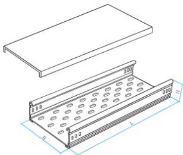
DJ型托盘式大跨距电缆桥架 Tray Type Long Span Cable Tray Model DJ (B型)
