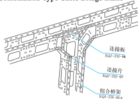
组合式电缆桥架垂直弯通及几种锯切示意图 Sketch map of Vertical Curved-Way and several Sawcut of Combination-Type Cable Bridge frame
