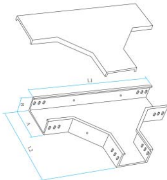
扁形水平等径三通 XQJ-C-3A Platoid Horizontal Equant T-joint Cable Tray
