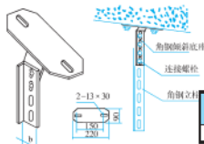
XQJ-H-03D角钢倾斜底座 Angle-Steel Tilt Base
