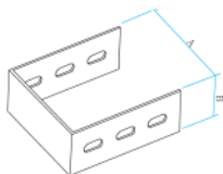
扁形水平等径弯通 XQJ-C-2A Platoid Horizontal Equant Elbow Joint Cable Tray Model XQJ-C-2A
