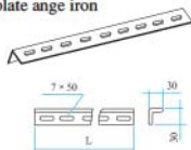
FJ-09花盘角铁 Faceplate ange iron
