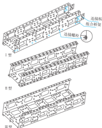
组合式直通桥架组装示意图 Installation Sketch Map of Combination-Type Straight-Way Bridgeframe
