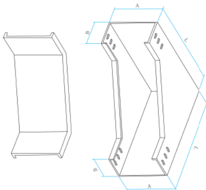
扁形水平等径下弯通 XQJ-C-2C Vertical Equant Lower Elbow Joint Cable Tray Model XQJ-C-2C
