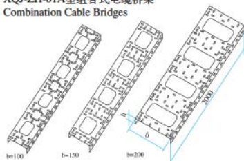
XQJ-ZH-01A型组合式电缆桥架 Combination Cable Bridges
