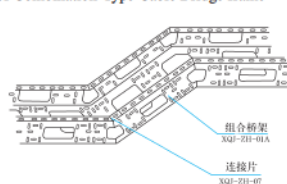
组合式电缆桥架垂直弯通及几种锯切示意图 Sketch map of Vertical Curved-Way and several Sawcut of Combination-Type Cable Bridge frame
