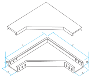
扁形水平等径弯通 XQJ-C-2A Platoid Horizontal Equant Elbow Joint Cable Tray Model XQJ-C-2A
