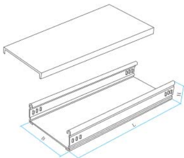
DJ型槽式大跨距电缆桥架 Channel Type Long Span Cable Tray Model DJ (B型)
