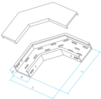
托盘式水平弯通 XQJ-P1-02 Tray Type Horizontal Elbow Joint Cable Tray Model XQJ-P1-02
