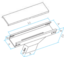
下边垂直等径三通 XQJ-C-3E Catadrome Side Vertical Equant T-joint Cable Tray
