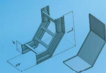
QJGHFF-T-05A型梯级式垂直上弯通
